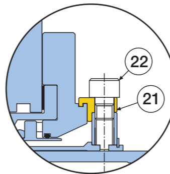
Setting Clip Details
